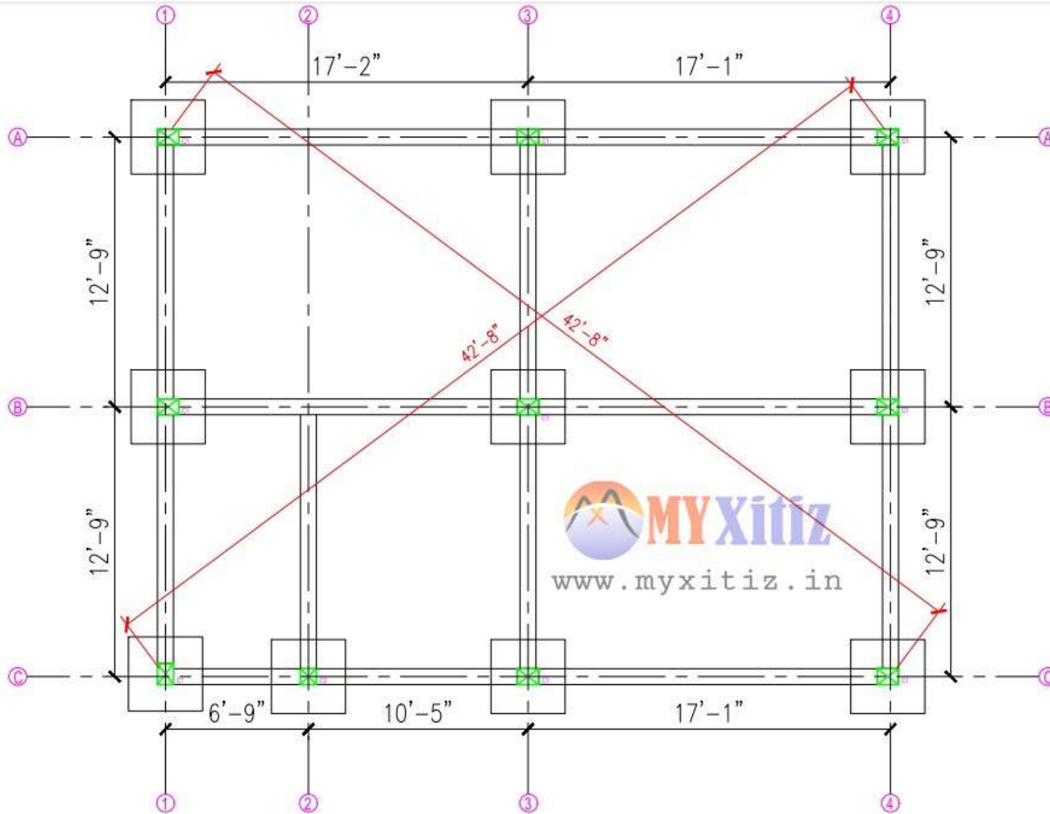
COLUMN LAYOUT & FOOTING PLAN
