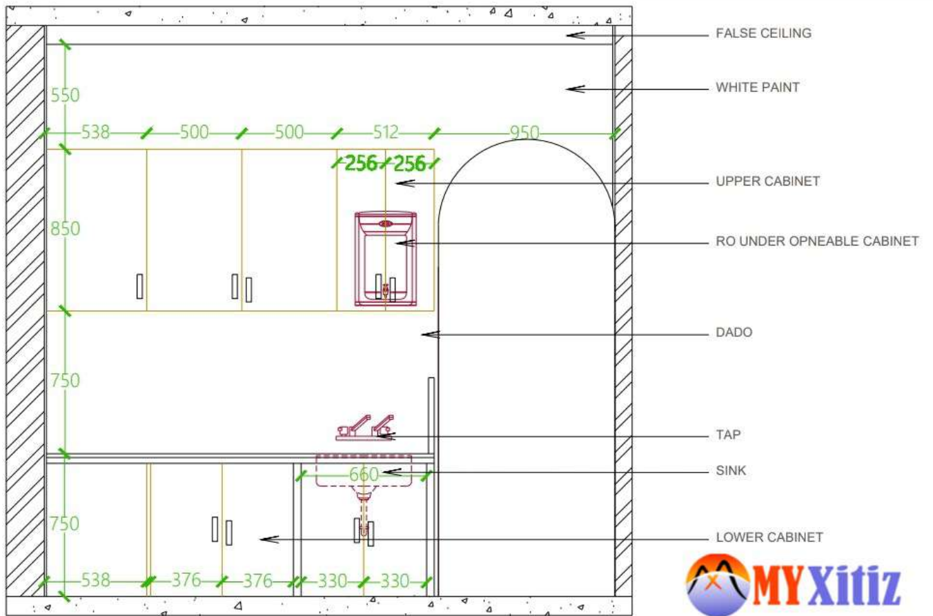
SECTION AT LL'
