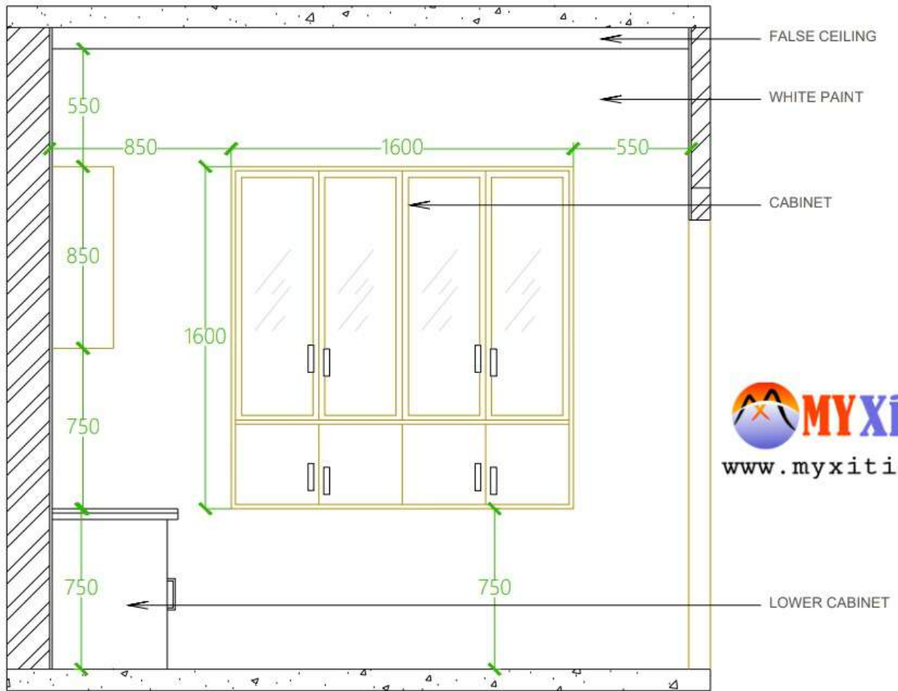
SECTION AT MM'
