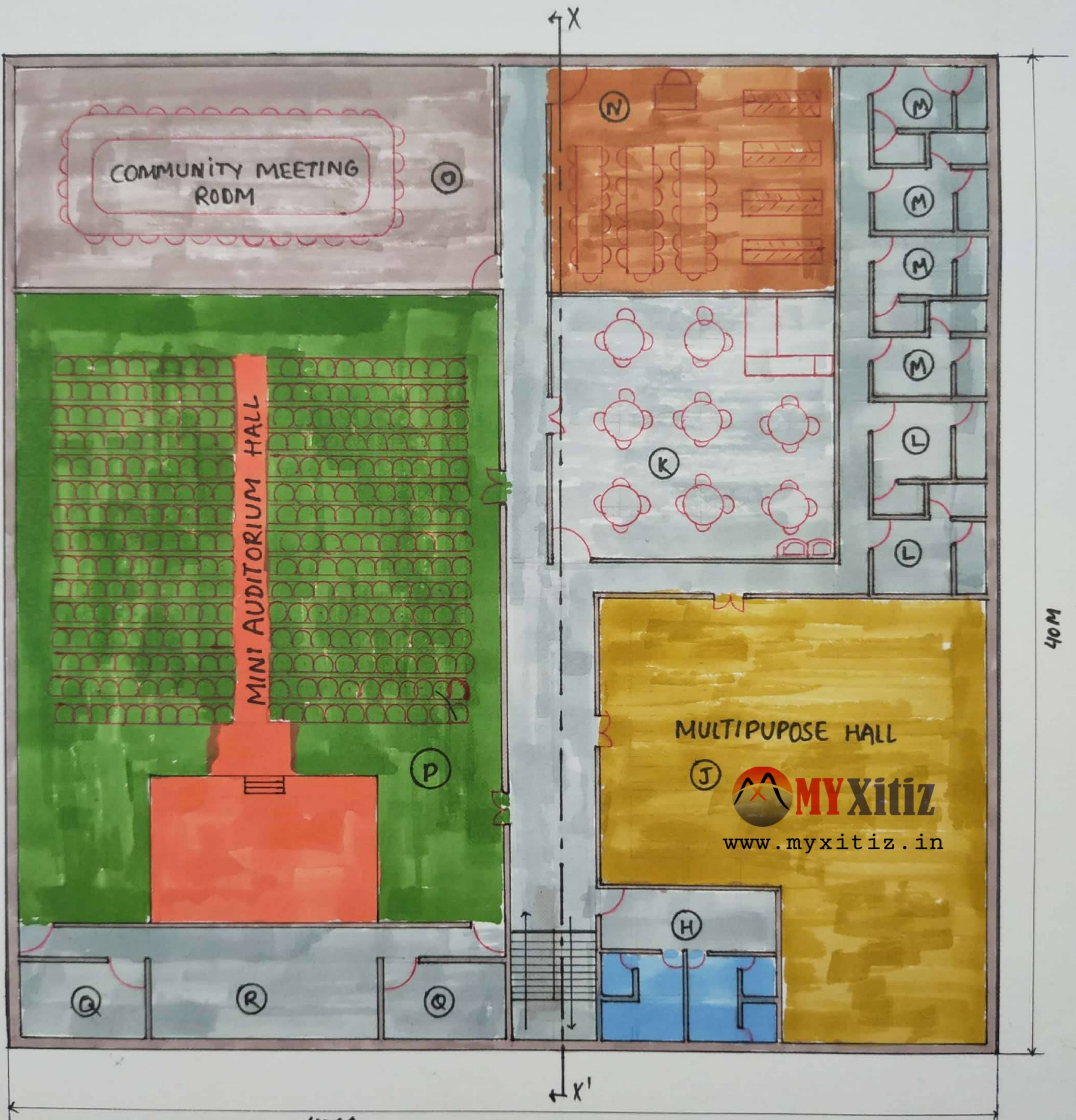
FIRST FLOOR PLAN
