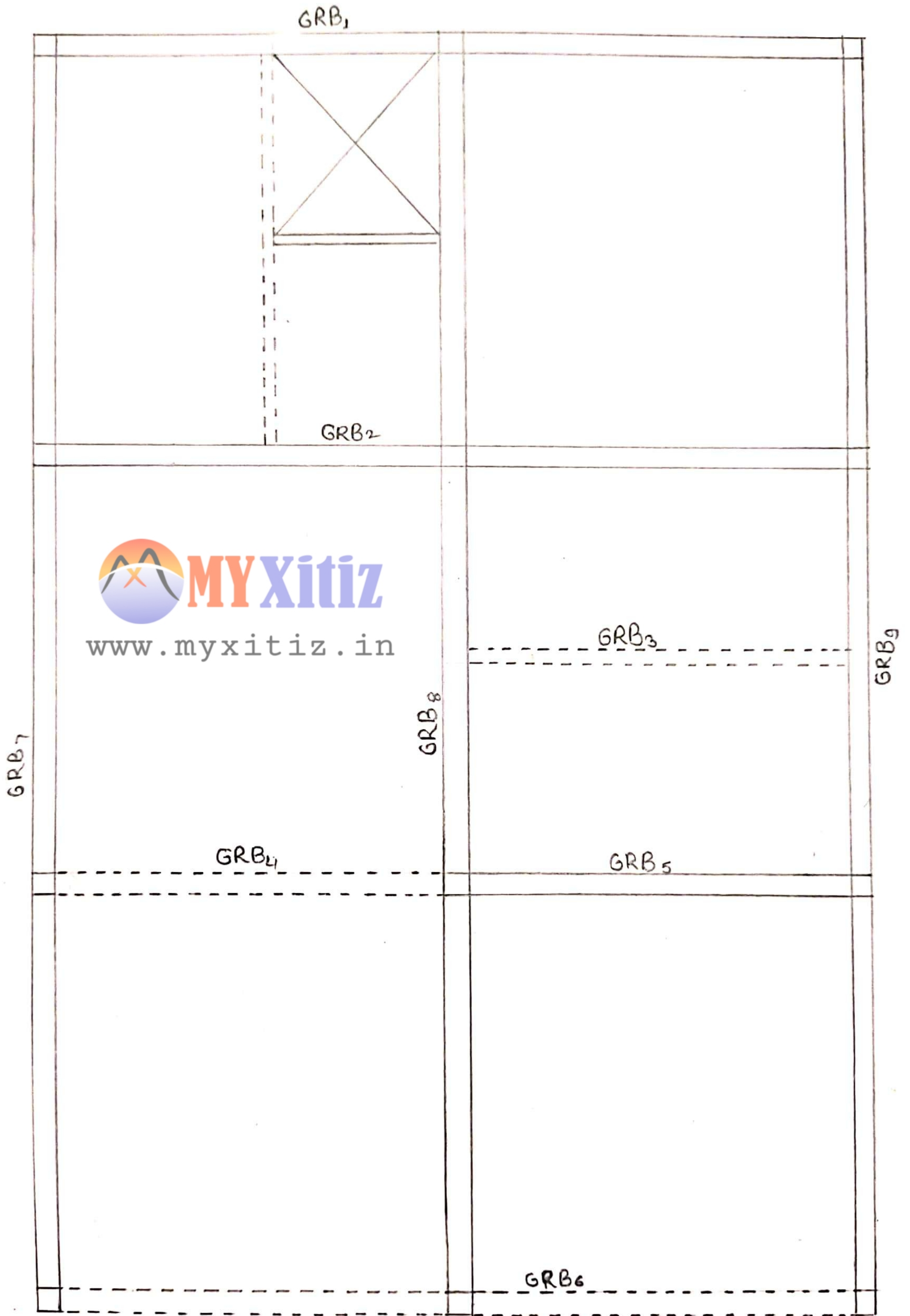
GROUND FLOOR BEAM LAYOUT
