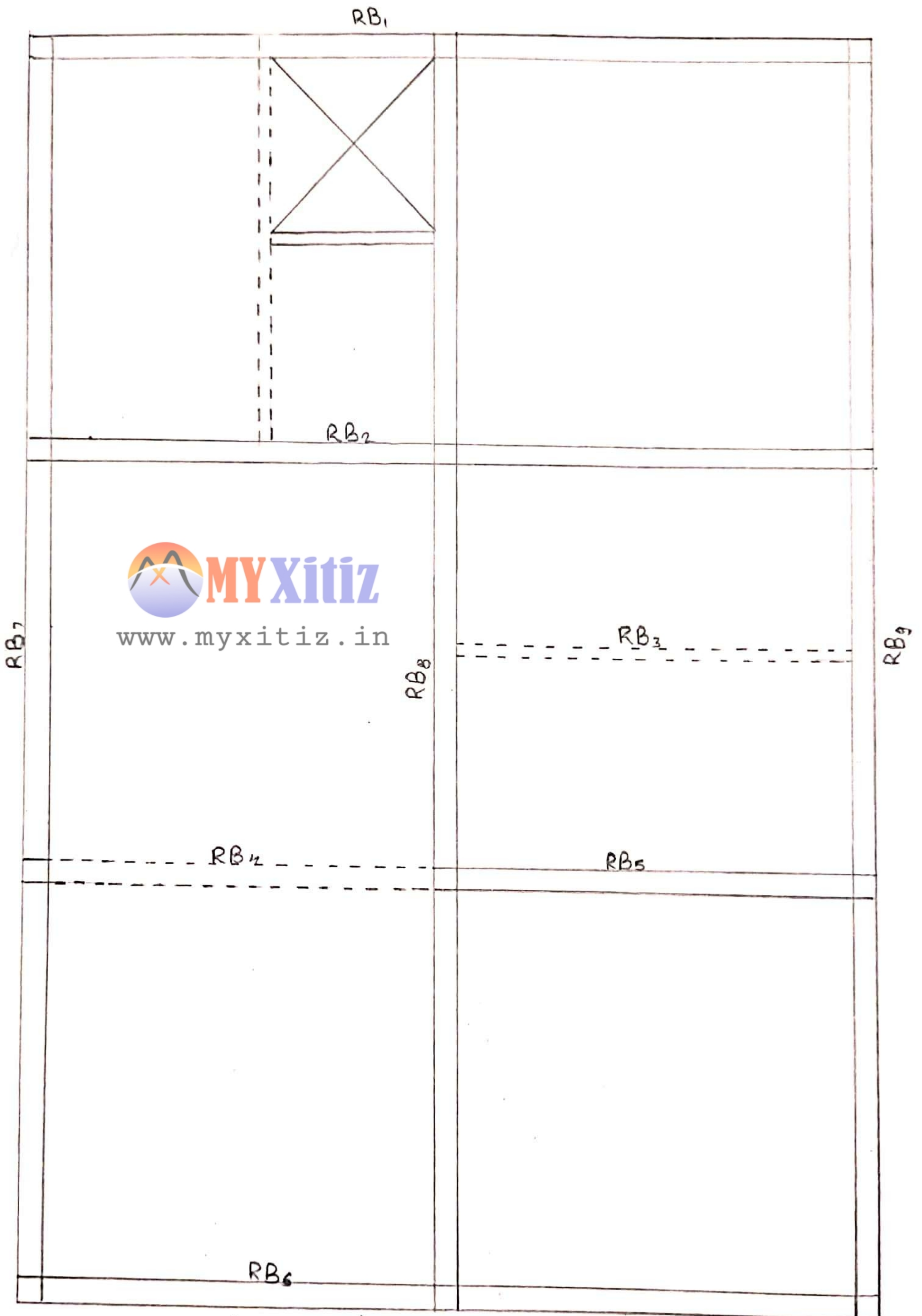
1 st AND 2 nd FLOOR BEAM LAYOUT
